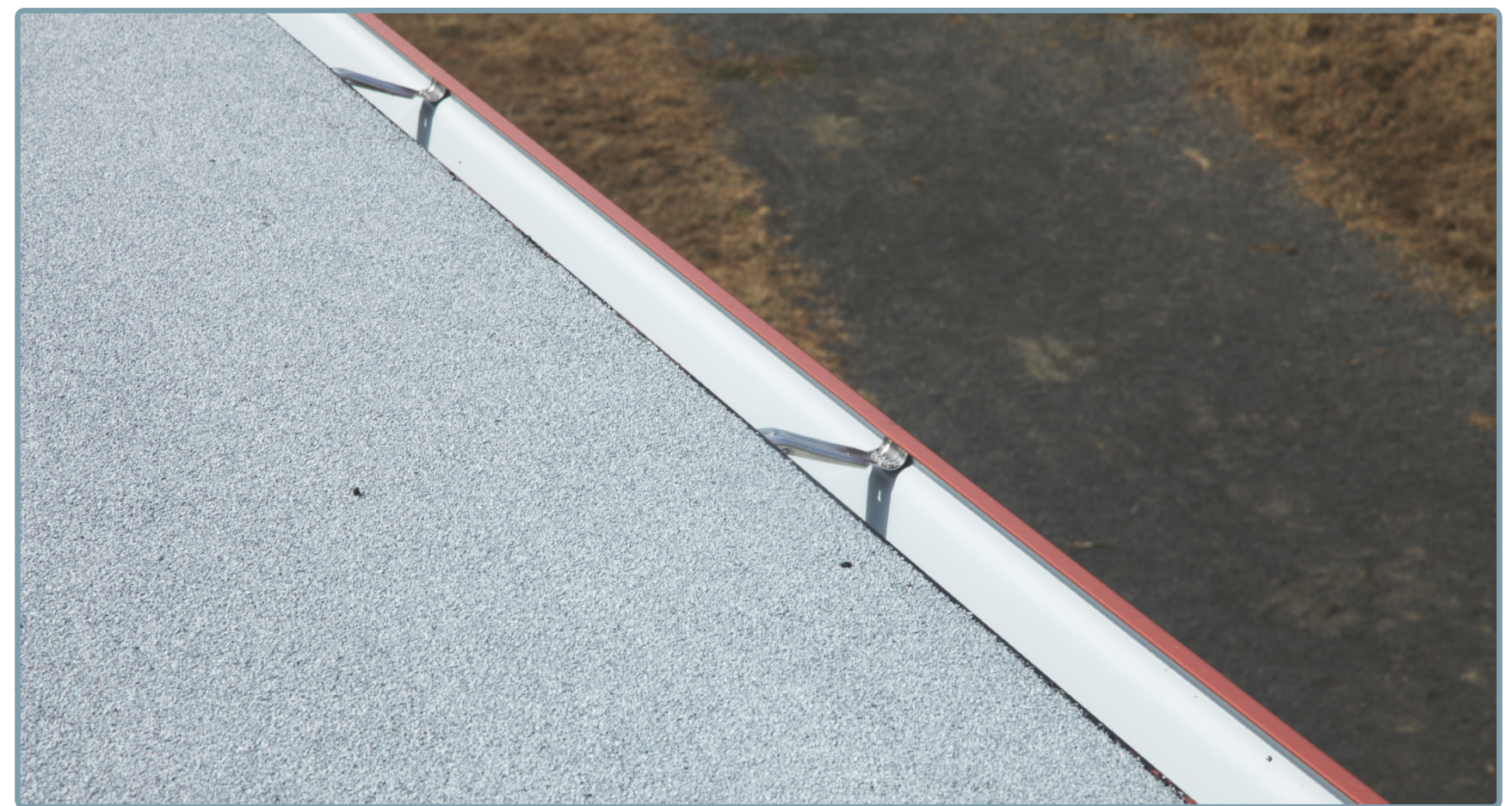
Installing plywood sheathing, new insulation, membrane roofing, vents and mechanical hoods.
